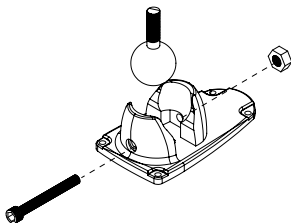
NEO 5A/6A/8A Metal wall-mount bracket (included)
